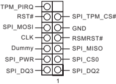
SPI_TPM_J1
